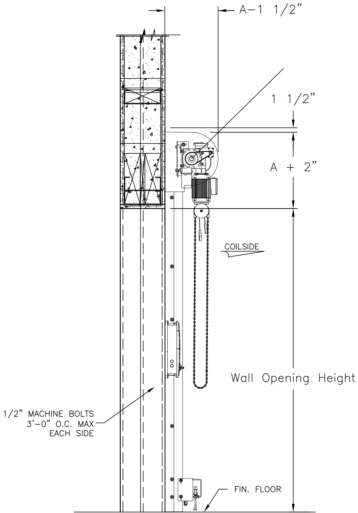
SECTION B-B
