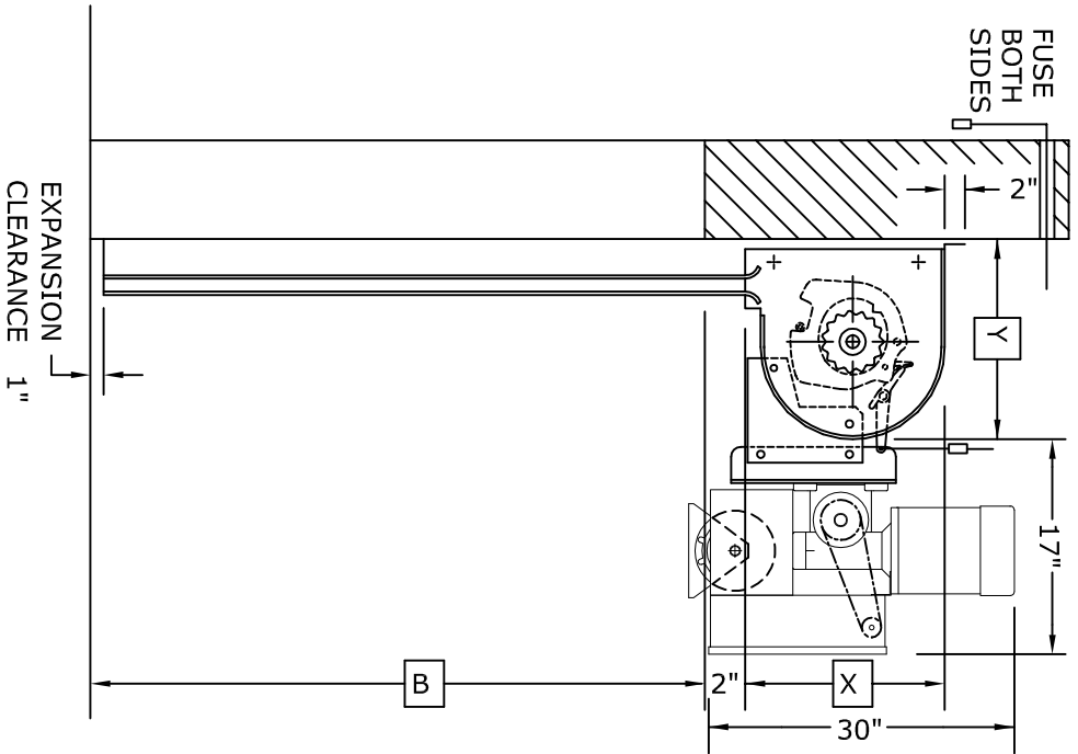
SIDE VIEW MOTOR OPERATED FIRE DOOR
