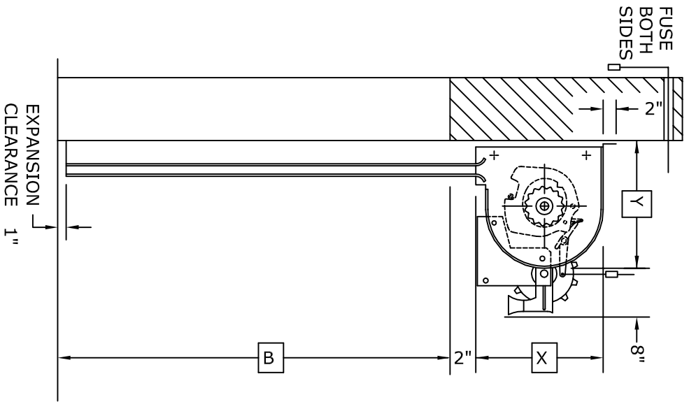
SIDE VIEW CHAIN HOIST OPERATED FIRE DOOR
