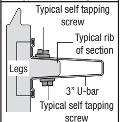
Side profile of a typical 3" u-bar attachment shown.
