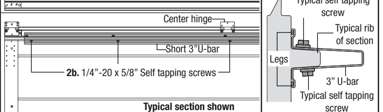
Side profile of a typical 3" u-bar attachment shown.
