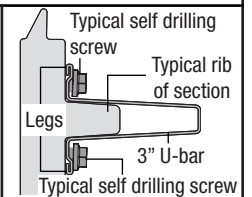
Typical top section shown
